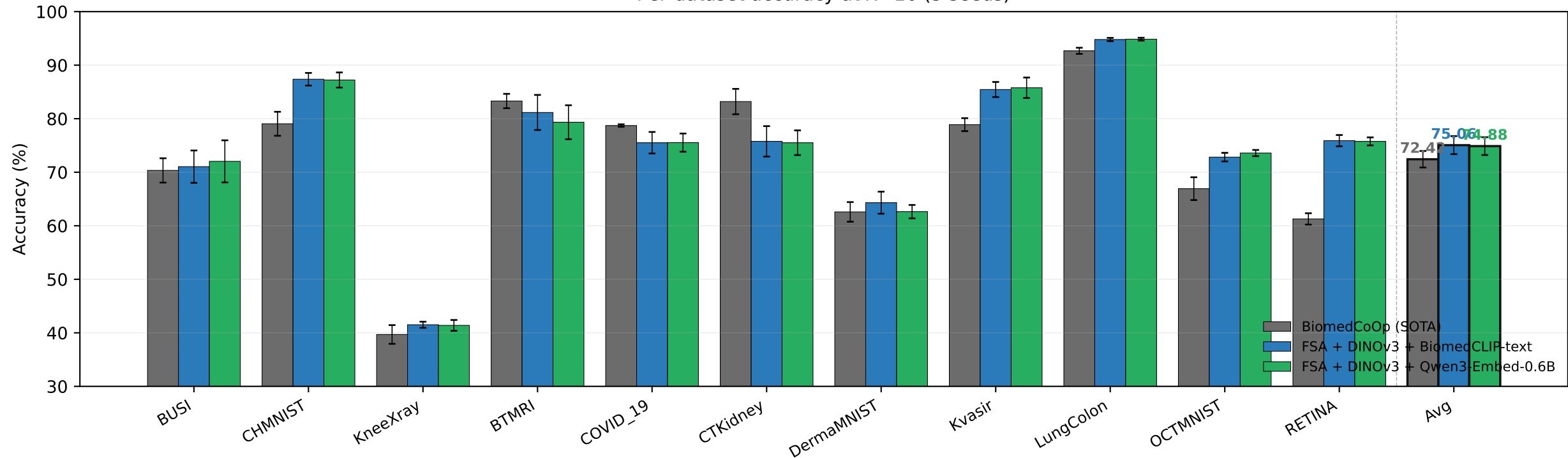
Per-dataset accuracy at K=16 (3 seeds)
