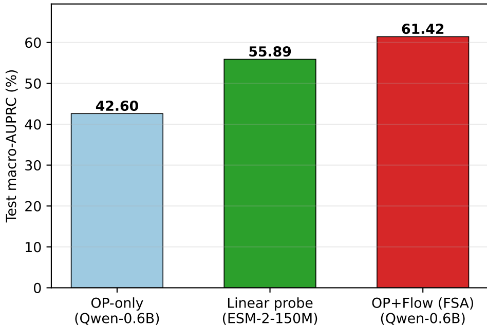
Full-train DeepLoc 2.0 Multi (N=21,948)
