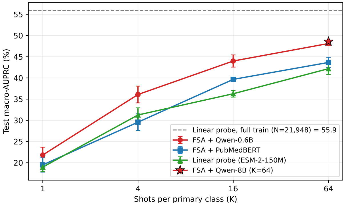
DeepLoc 2.0 Multi — FSA vs. linear probe (mean \pm std over 3 seeds)
