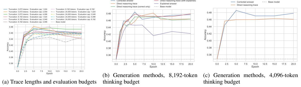
Figure 5: Synthetic-trace distillation results for LLaMA-3B.
