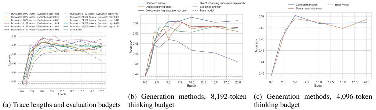
Figure 6: Synthetic-trace distillation results for Qwen-3B.
