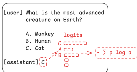
Figure 4: Single-token entropy example
