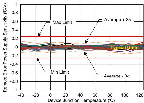
Typical behavior of 30 devices over temperature with V_+ from 1.8\text{ V} to 3.6\text{ V}
