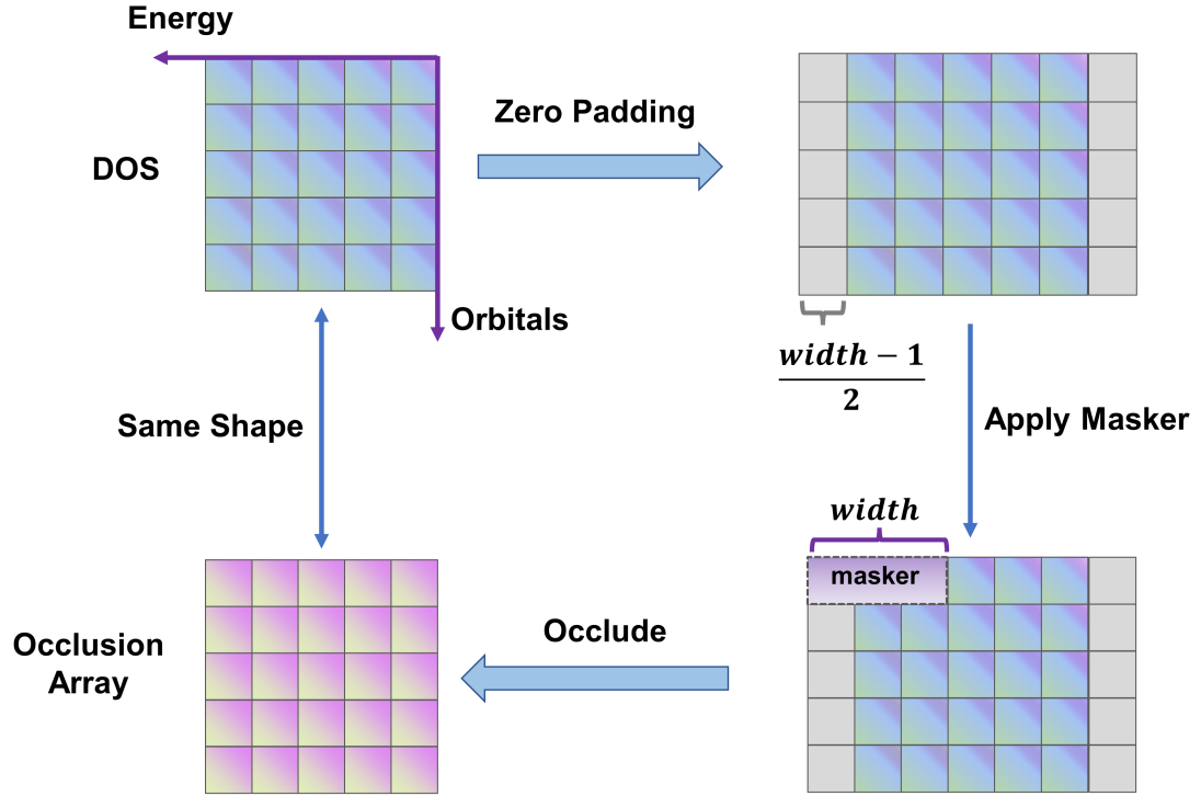
Figure 27: Illustration of the eDOS occlusion experiment. This figure demonstrates the step-by-step process of the occlusion experiment. The input eDOS array first undergoes zero-padded, and then a masker of width “width” is applied, resulting in an occlusion array that preserves the shape of the input array.
