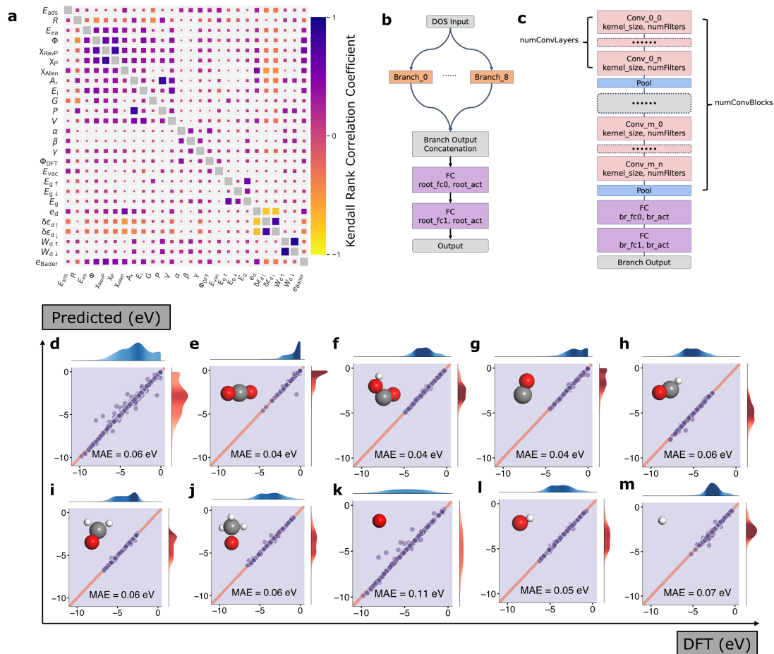
Figure 2: CNN for electronic density of states. a. Kendall rank correlation coefficient map illustrating the correlation between adsorption energy and other electronic and elementary descriptors. Definitions of the notations are provided in Supplementary section 2.2. b-c. Architectural of (b) the root and (c) each branch of the CNN model. The architecture stays consistent across individual branches. d-m. Parity plots demonstrating the performance of the CNN model across nine adsorbates: (d) all adsorbates, (e) \text{CO}_2 , (f) \text{COOH} , (g) \text{CO} , (h) \text{CHO} , (i) \text{CH}_2\text{O} , (j) \text{OCH}_3 , (k) \text{O} , (l) \text{OH} , and (m) \text{H} . The augmentation data are not displayed in these plots, nor included in MAE evaluations. Kernel density estimate results are shown along the top and right sides of the main plot, representing DFT calculations and CNN model prediction distributions, respectively.
