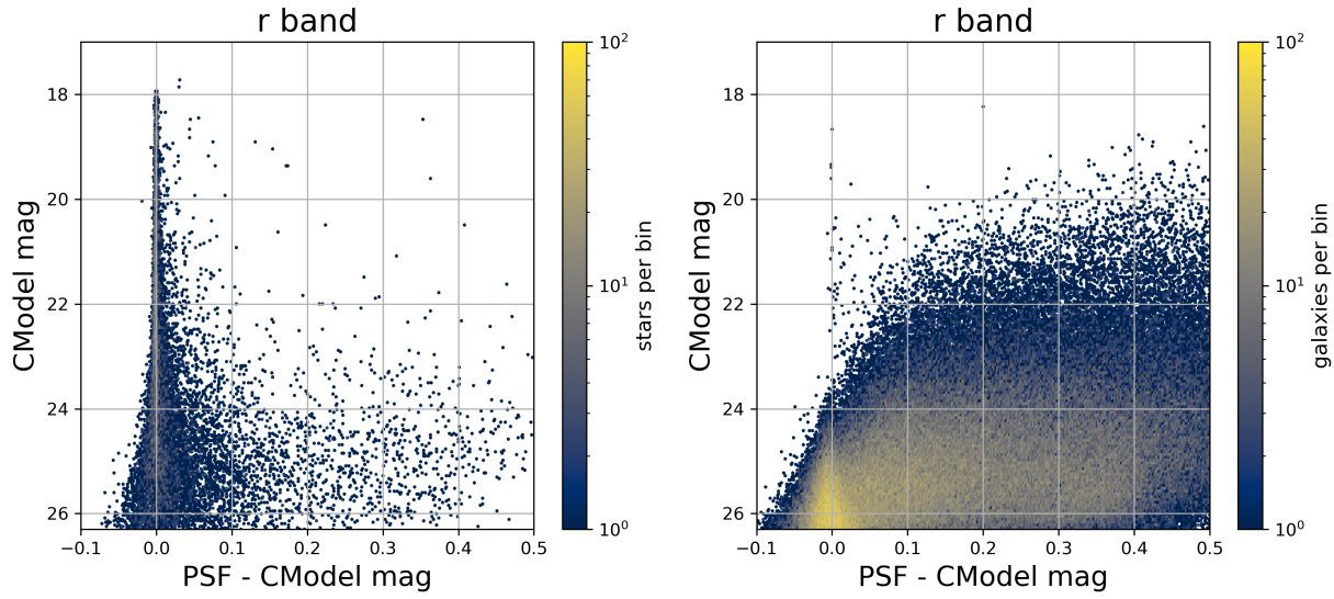
Figure 8. The panels show the \Delta m vs. m_{\text{CModel}} distributions for unresolved (left) and resolved (right) objects classified using HST labels. Note that some objects in the left panel appear clearly resolved by Rubin ( \Delta m > 0.05 ), even for r < 24 (see §2.5), and that galaxies (right panel) dominate the region around \Delta m \sim 0 at the faint end ( r > 24 ). Quantitative modeling of these two-dimensional distributions is at the core of the star-galaxy separation method discussed here.
