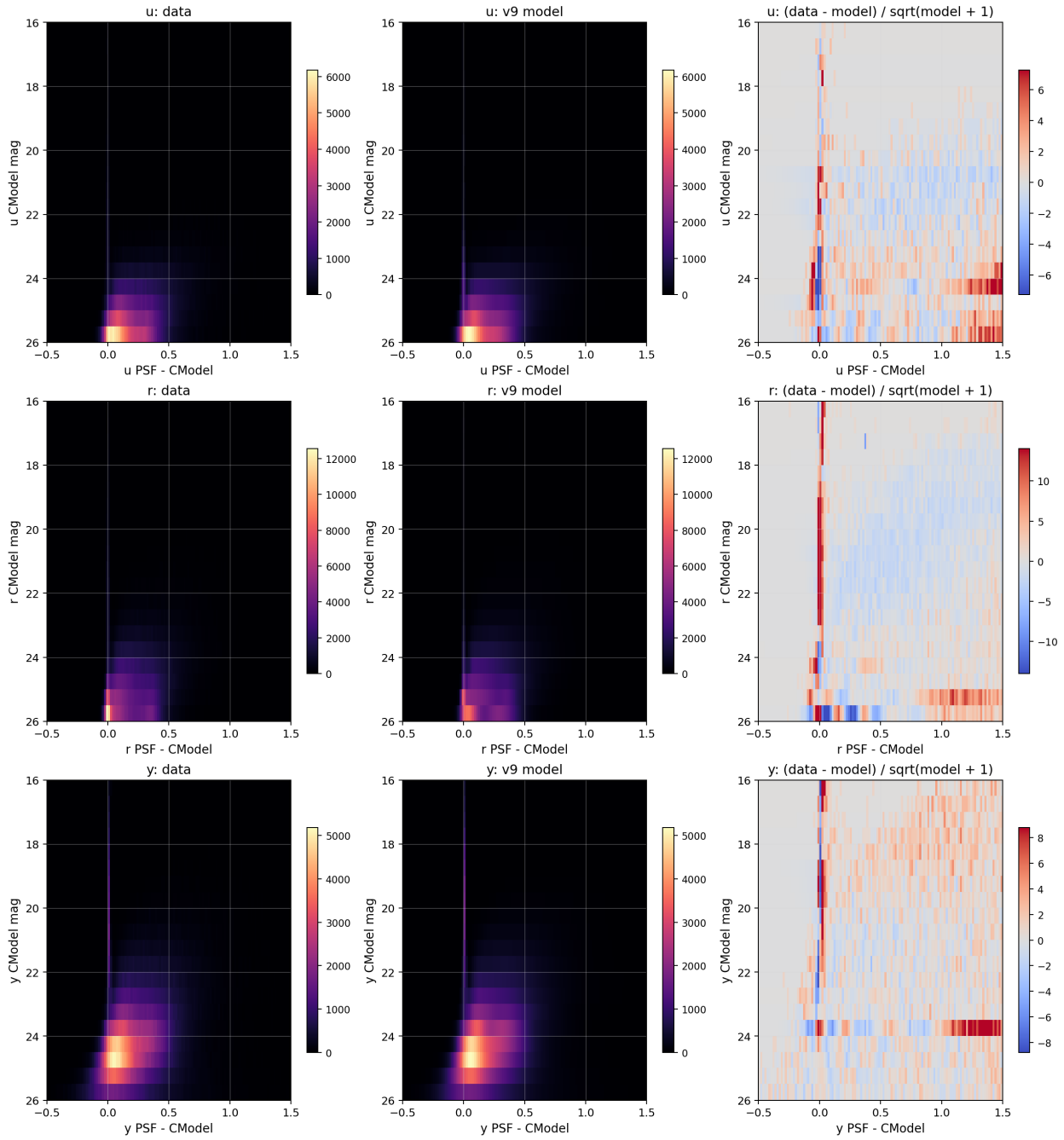
Figure 11. Two-dimensional comparison of the observed (left), modeled (center), and residual (right) source density in the \Delta m vs. m_{\text{CModel}} plane. The small residuals demonstrate that the constrained mixture model provides an adequate description of the data across the full magnitude range.
