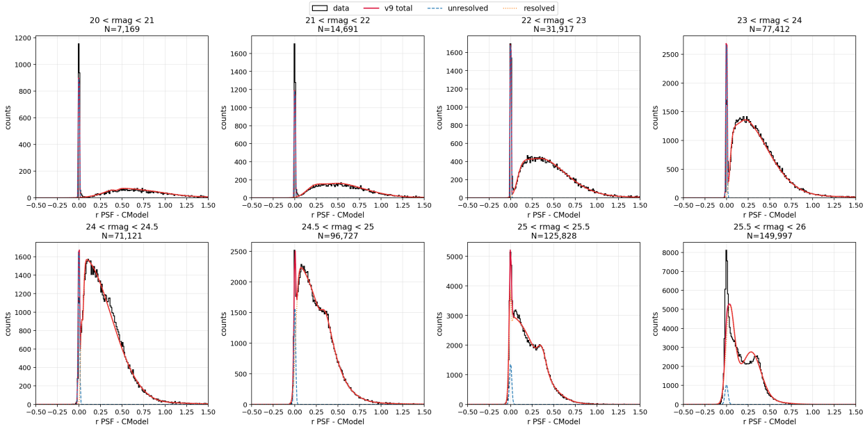
Figure 10. Observed \Delta m histograms (black) and fitted mixture models (red) for the r-band in each CModel magnitude bin. The unresolved Gaussian component is shown as a blue dashed line and the resolved log-normal components as orange dotted lines.
