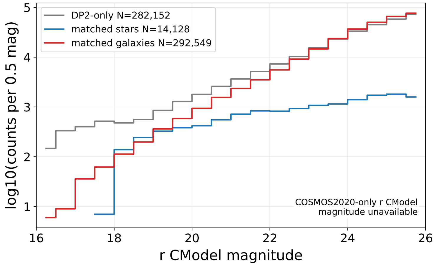
Counts vs r magnitude
