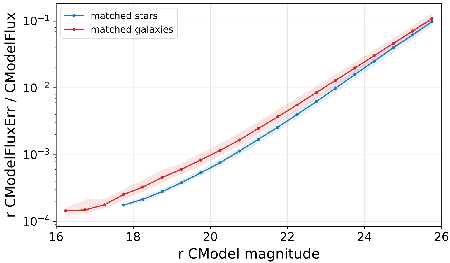
Relative model flux uncertainty
