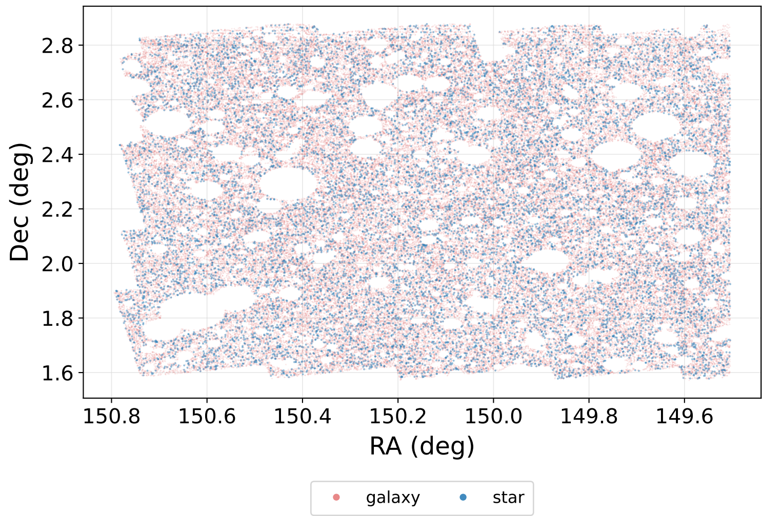
Matched COSMOS2020-DP2 sample
