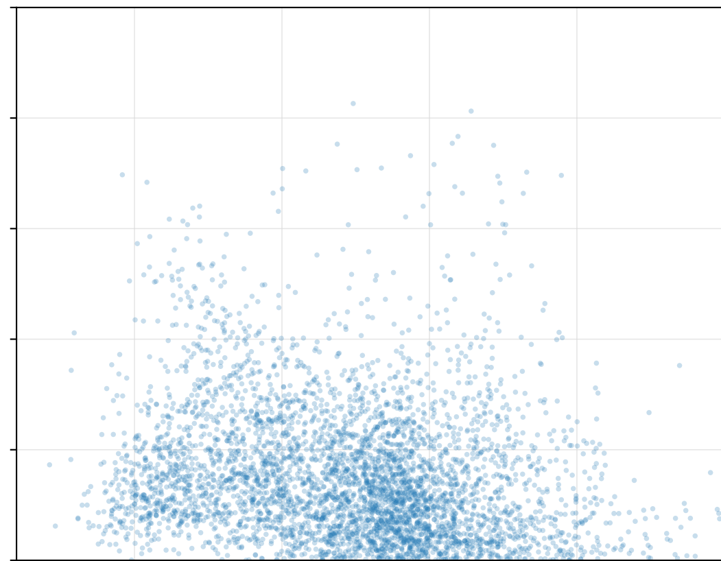
SG: truth star, class galaxy N=4,419
