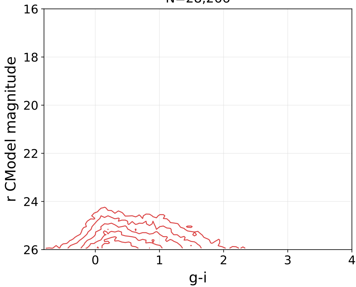
GS: truth galaxy, class star N=28,266
