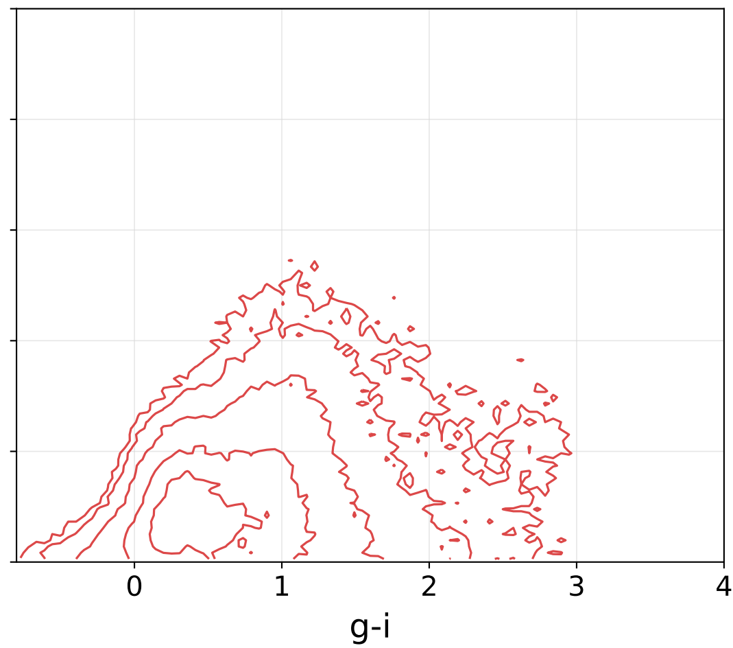
GG: truth galaxy, class galaxy N=256,460
