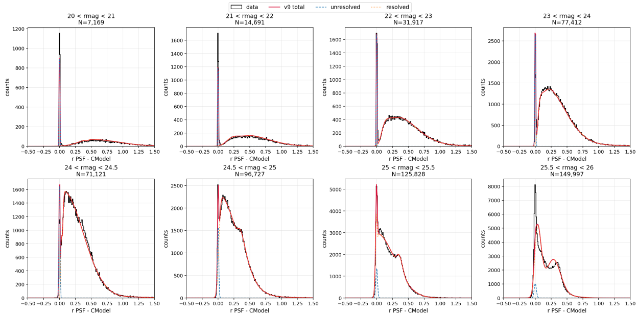
Figure 6. Observed \Delta m histograms (black) and fitted mixture models (red) for the r-band in each CModel magnitude bin. The unresolved Gaussian component is shown as a blue dashed line and the resolved skew-normal components as orange dotted lines.
