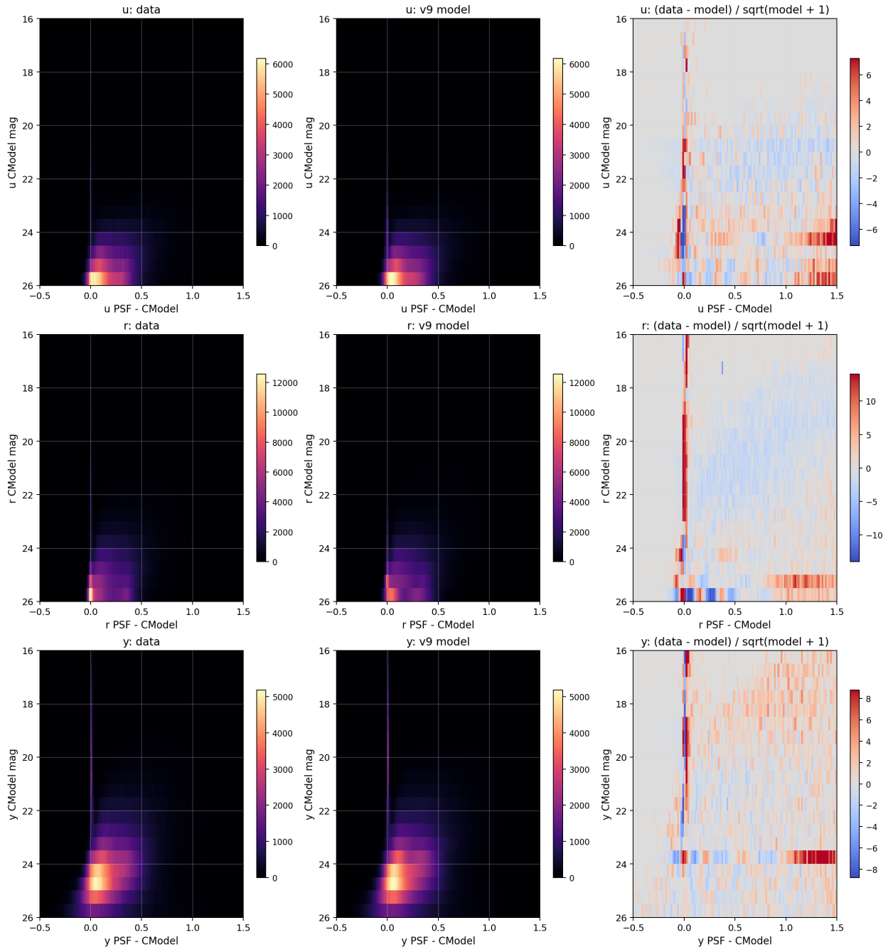
Figure 7. Two-dimensional comparison of the observed (left), modeled (center), and residual (right) source density in the \Delta m vs. m_{\text{CModel}} plane. The small residuals demonstrate that the constrained mixture model provides an adequate description of the data across the full magnitude range.
