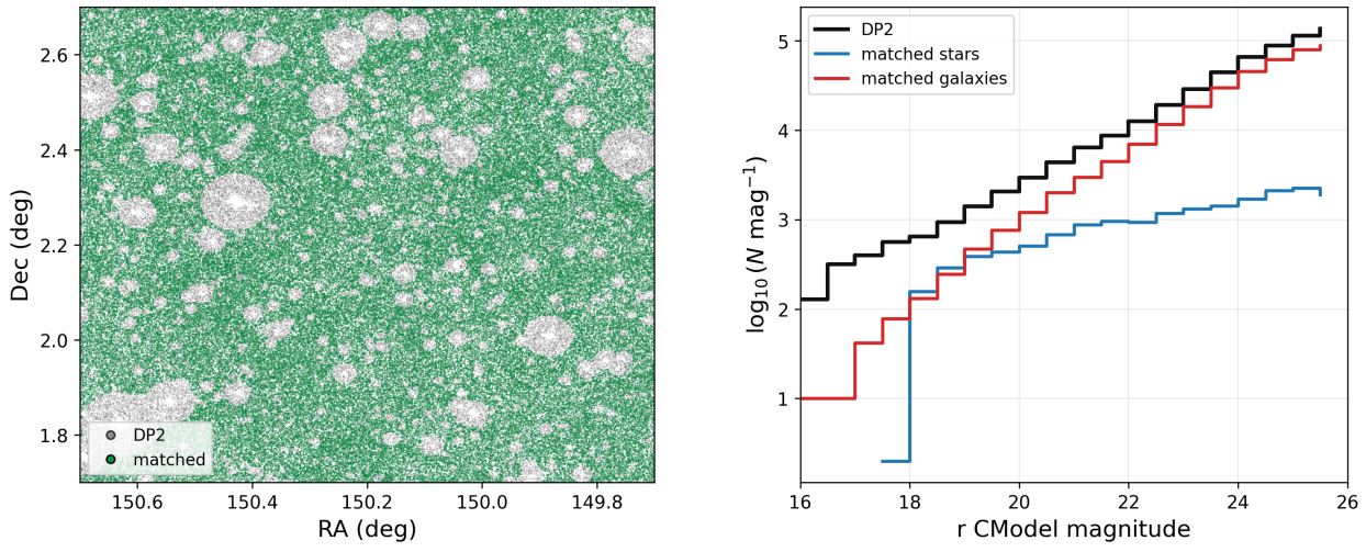
Figure 1. COSMOS/COSMOS2020 matched sample overview. The primary sample is selected using uncorrected r-band CModel magnitude, while colors are dust-corrected where applicable. XXX: SPLIT THIS FIGURE INTO 2 FIGURES; top panel: remove title; instead of galaxy and stars, show all DP2 sources in one color and overplot matches in other color; remove legend below (this information needs to go into caption; bottom panel: multiply counts by 2 to get unit to be per mag; remove title and text in the bottom right; HOW CAN RED LINE BE ABOVE GRAY LINE? It's probably some error in effective area or such... We don't need the third panel.
