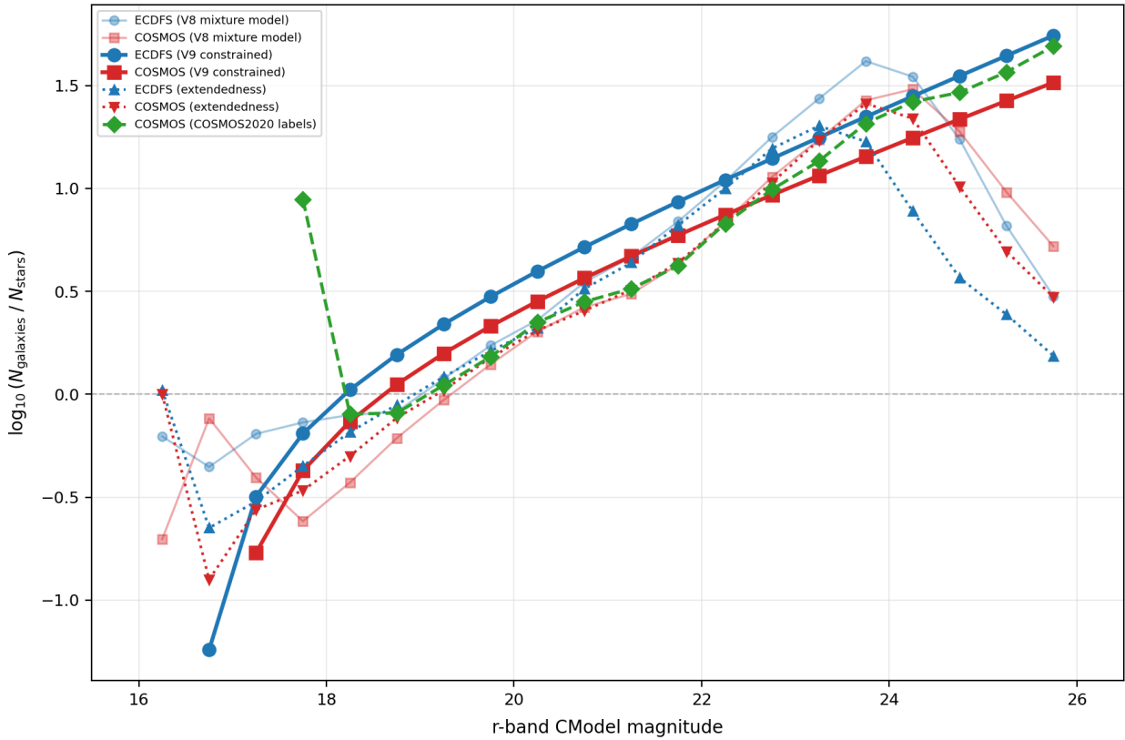
Figure 5. Galaxy-to-star count ratio \log_{10}(N_{\text{gal}}/N_{\text{star}}) vs. r-band CModel magnitude. The unconstrained mixture model (V8, faded curves) exhibits a spurious turnover at m \gtrsim 24 due to the unresolved Gaussian absorbing galaxy flux. The constrained model (V9, bold curves) recovers the expected monotonically increasing ratio, in good agreement with the COSMOS2020 truth labels (green dashed). Dotted lines show the Rubin extendedness -based classification for comparison.
