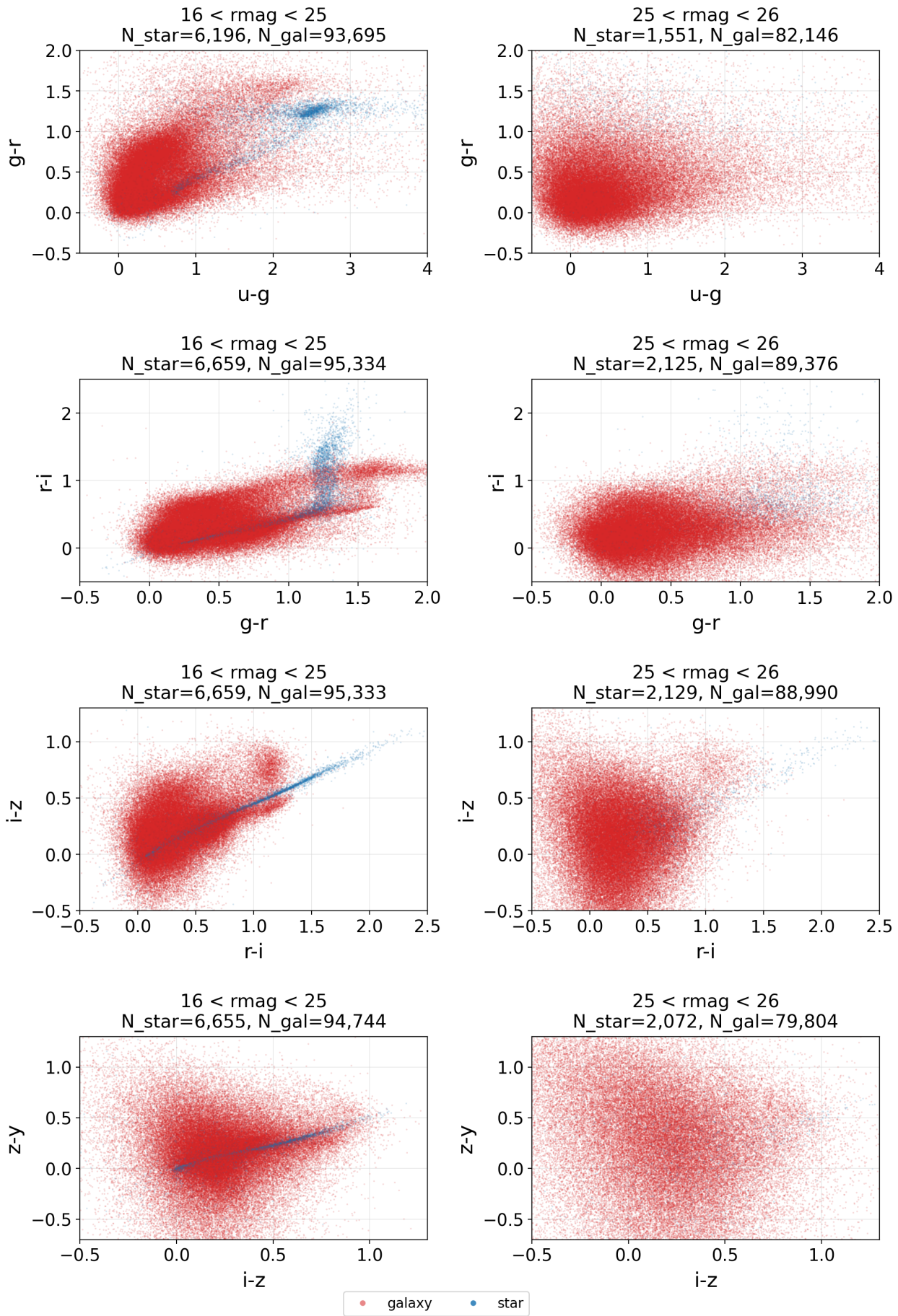
Figure 3. Similar to Figure 2, except that data are split by r-band CModel magnitude to show deterioration close to the faint magnitude limit (left: 16 < \text{rmag} < 25 ; right: 25 < \text{rmag} < 26 ).
