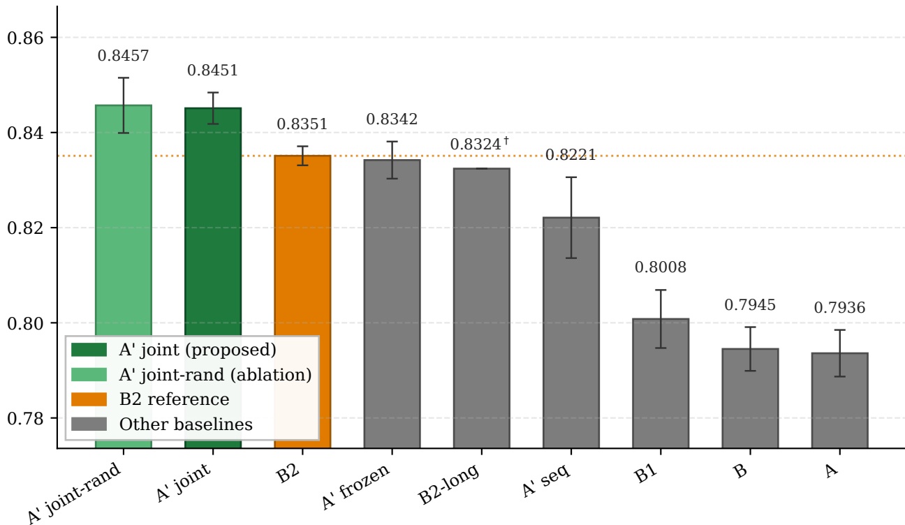
mAP50 (CITRA-3D-Real test set)
