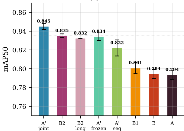
(a) mAP50
