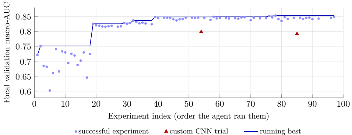
Figure 3: The agent’s discovery trajectory over its successful experiments. Phase 1 (idx 1–18): cold-start exploration, the agent oscillates between 0.60 and 0.75 while it settles the architecture and augmentation family. Phase 2 (idx 19–38): a sharp jump to \geq 0.82 once the agent starts systematically sweeping mel-spectrogram parameters. Phase 3 (idx 39 onward): fine refinement and convergence, plateauing at the best run 0.8533 ( topdb_40_optimal_preprocessing , idx 78). The two red triangles are the only two custom-CNN runs the agent ever tried.
