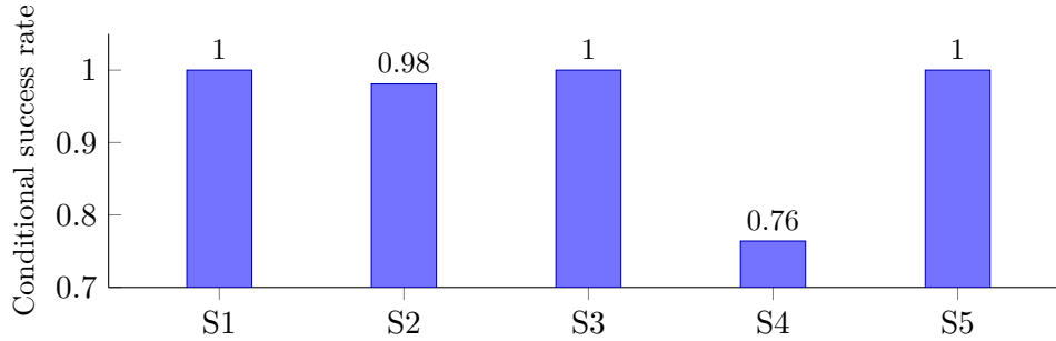
Figure 2: Stage-conditional success rates P(\text{stage}_k \mid \text{stage}_{k-1}) across the agent’s five pipeline stages. The drop at S4 (training completion, 0.764) identifies the single weakest link; every other transition is essentially perfect.
