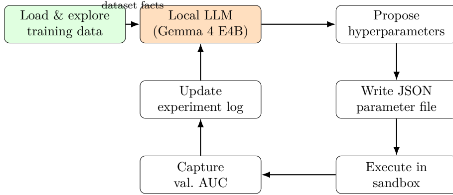
Figure 1: The closed explore–propose–generate–execute–evaluate–analyse–iterate loop. The green node runs once at startup; the dataset facts it produces are then prepended to every prompt the LLM receives, so each proposal is grounded in real data structure. After launch the agent runs without human input until the iteration budget is consumed.
