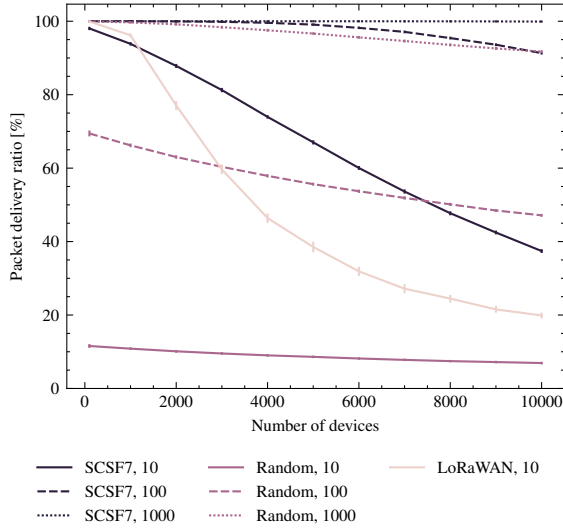
Fig. 3. Network packet delivery ratio for an increasing number of devices. Labels indicate the scenario and the number of deployed gateways. LoRaWAN's number of gateways is limited to 10 to match a city-wide deployment size [13].
