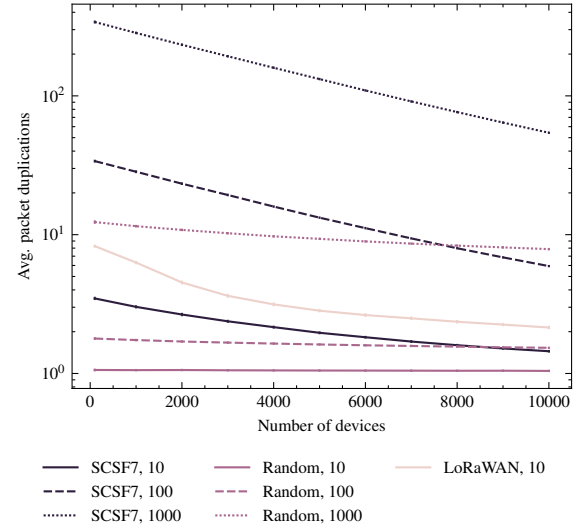
Fig. 4. Average number of duplicated receptions per successful packet for an increasing number of devices. Labels indicate the scenario and the number of deployed gateways. LoRaWAN's number of gateways is limited to 10 to match a city-wide deployment size [13].
