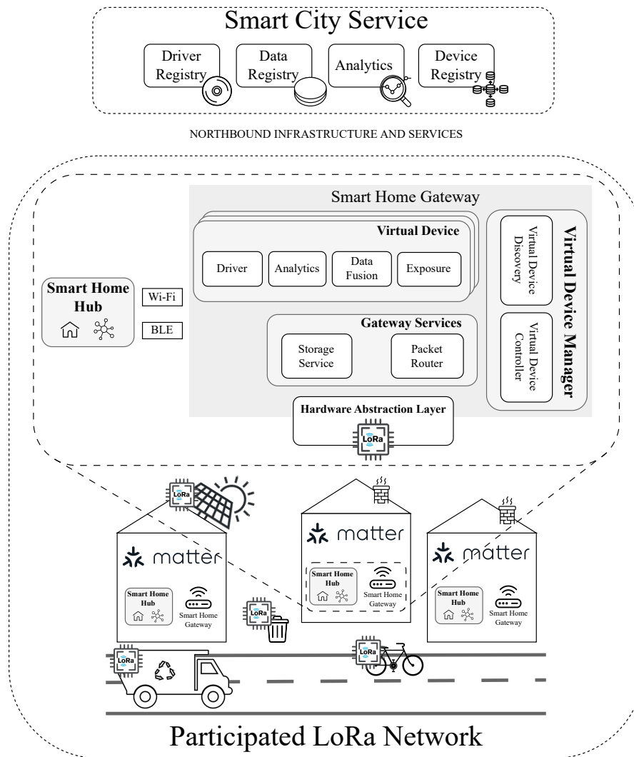
Fig. 2. Pluggable software architecture of the Smart Home Gateway capable of dynamic loading of device specific drivers (Virtual Devices) handling data synchronization, (pre)processing and exposure to local and/or global services. The SHG can interact with smart city services via northbound interfaces, and integrate locally with Smart Home products by exploiting standard Matter interfaces.
