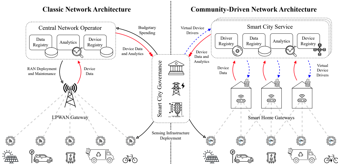
Fig. 1. On the left side is shown a single cell in a classic LPWAN architecture [3], while on the right is shown our participatory, decentralized LoRa network. Compared to a classic architecture, our Smart Home Gateways can be installed into citizens homes to foster a densification of receivers while providing participants direct access to locally sensed information and relieving municipalities from the cost of deploying and managing the infrastructure.
