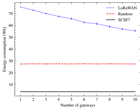
Fig. 5. Total energy consumption [Wh] of 10000 (i.e. 118 dev/km 2 ) LoRa transceivers for an increasing number of gateways. SCSF7 and Random are compared to a plausible LoRaWAN urban deployment, usually not larger than of 10 gateways [13].
