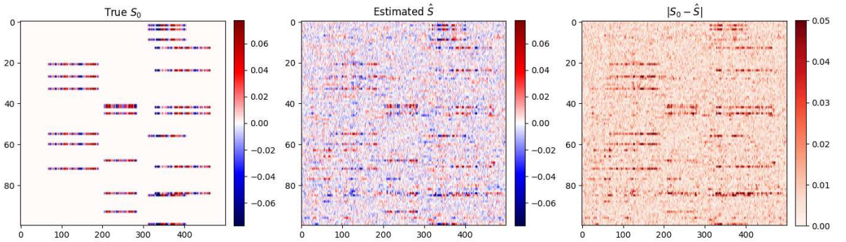
RUN2_ADMM_BASELINE_MISMATCH — DIAGNOSTICS
