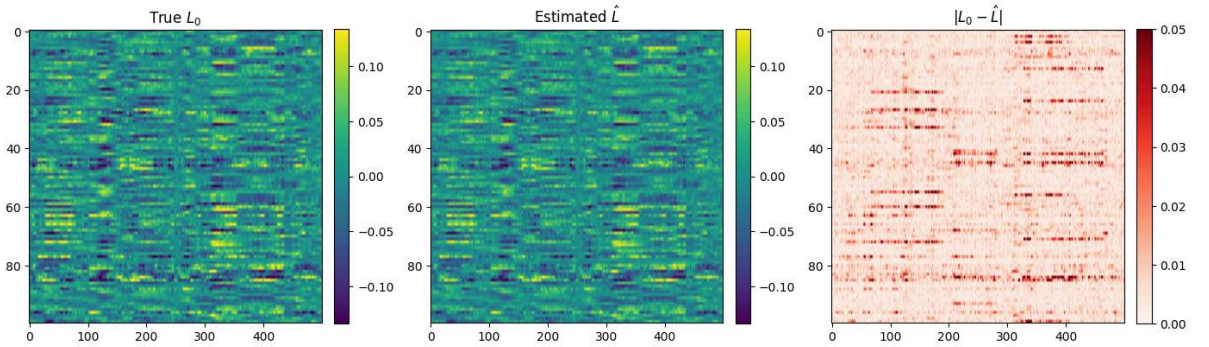
RUN2_ADMM_BASELINE_MISMATCH — SPARSE
