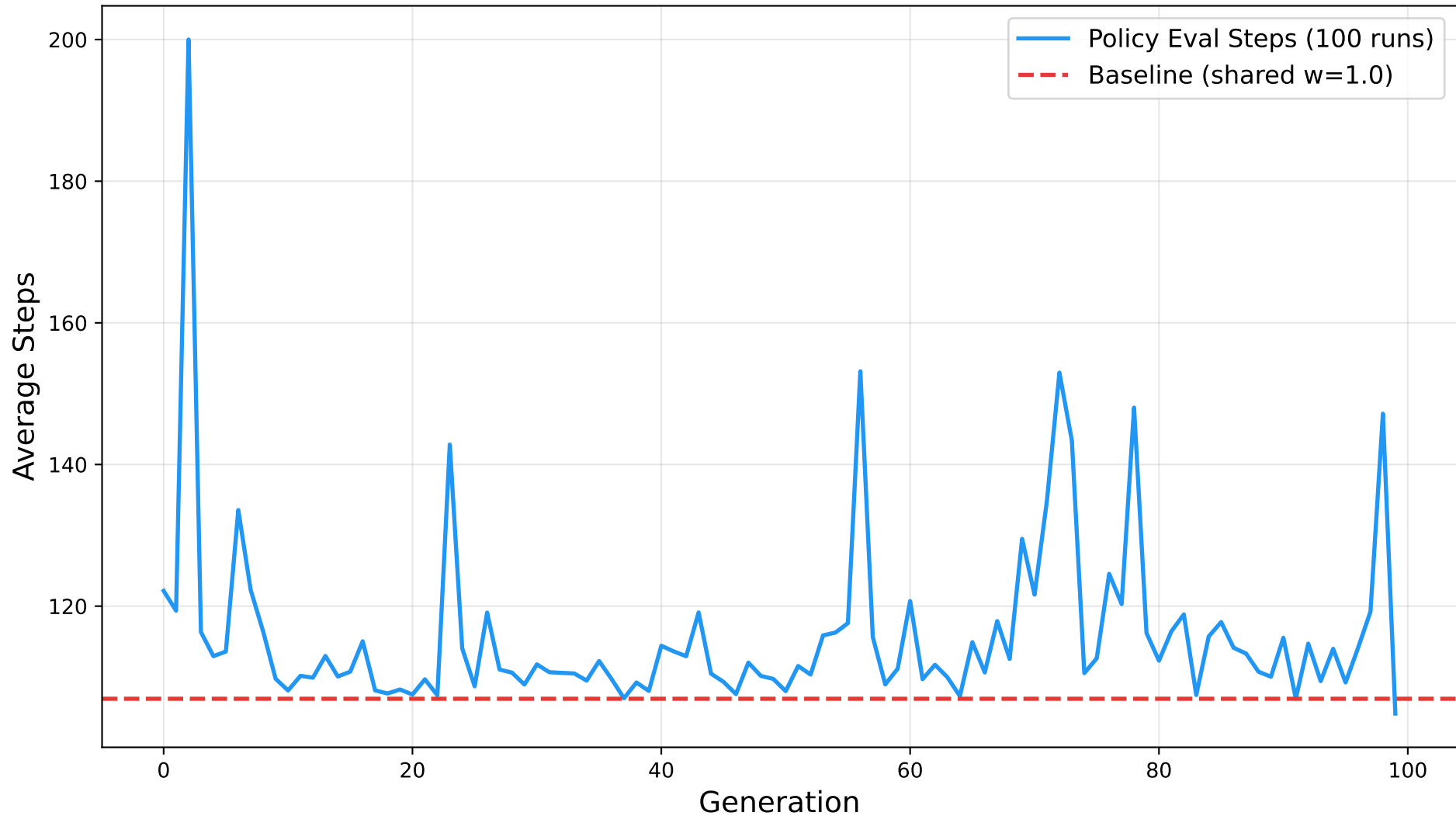
ES Weight Training — Steps per Generation
