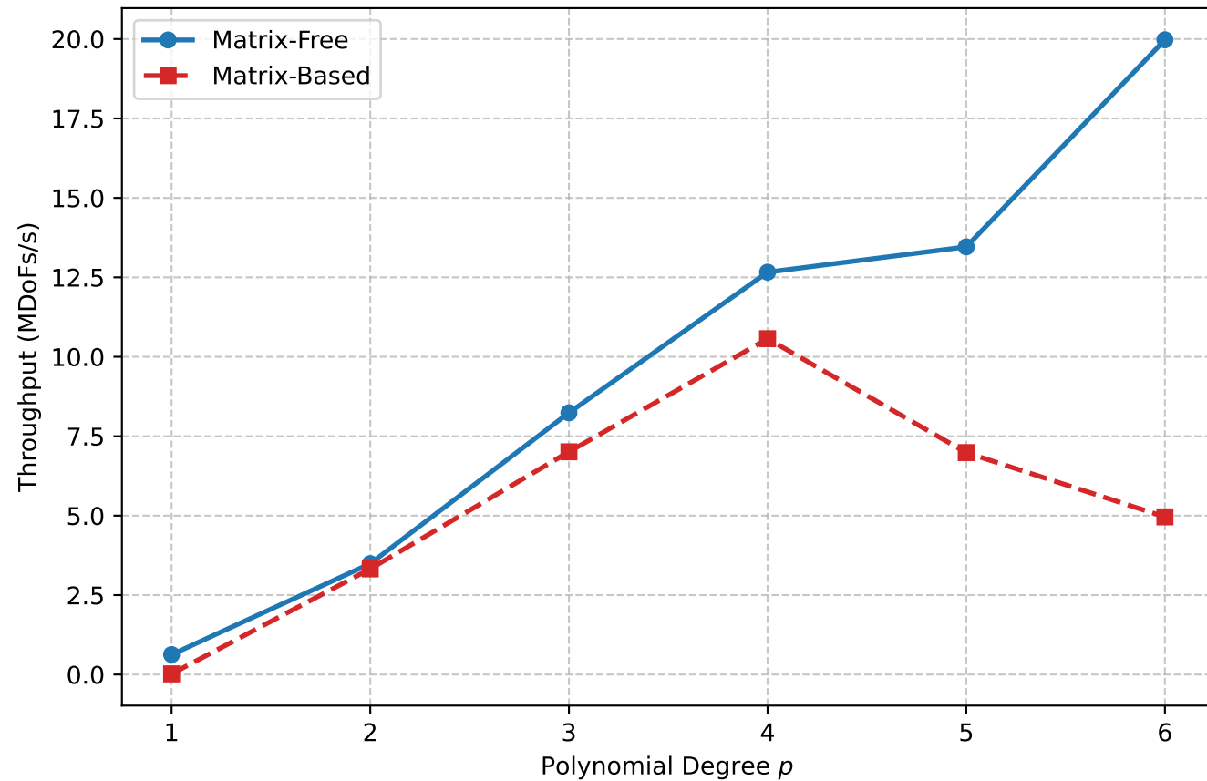
Throughput vs Polynomial Degree (56 Cores)
