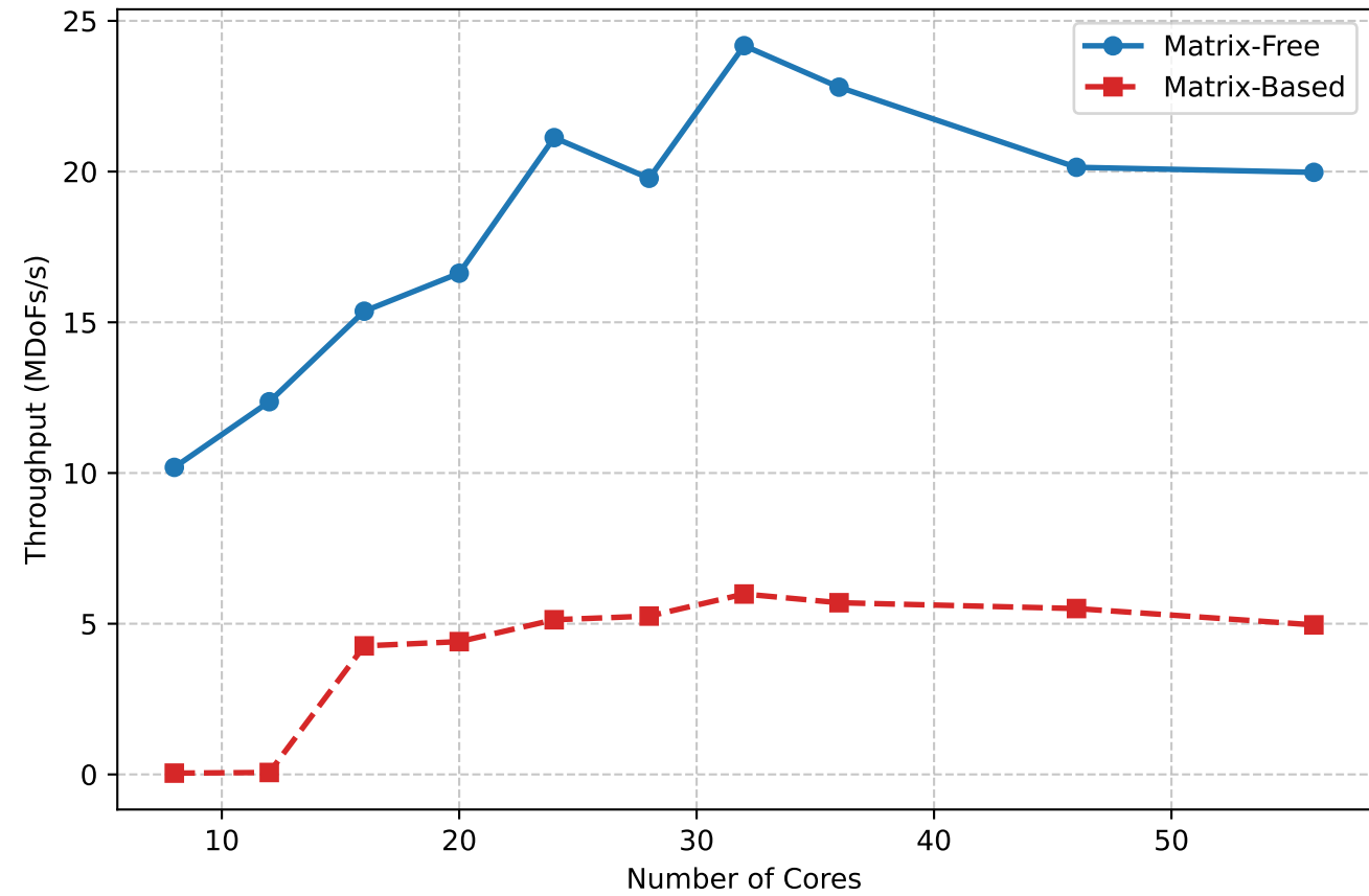
Throughput Scaling (Degree p = 6 )
