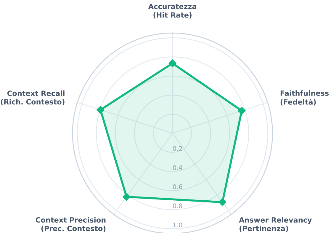
RAG Graph
