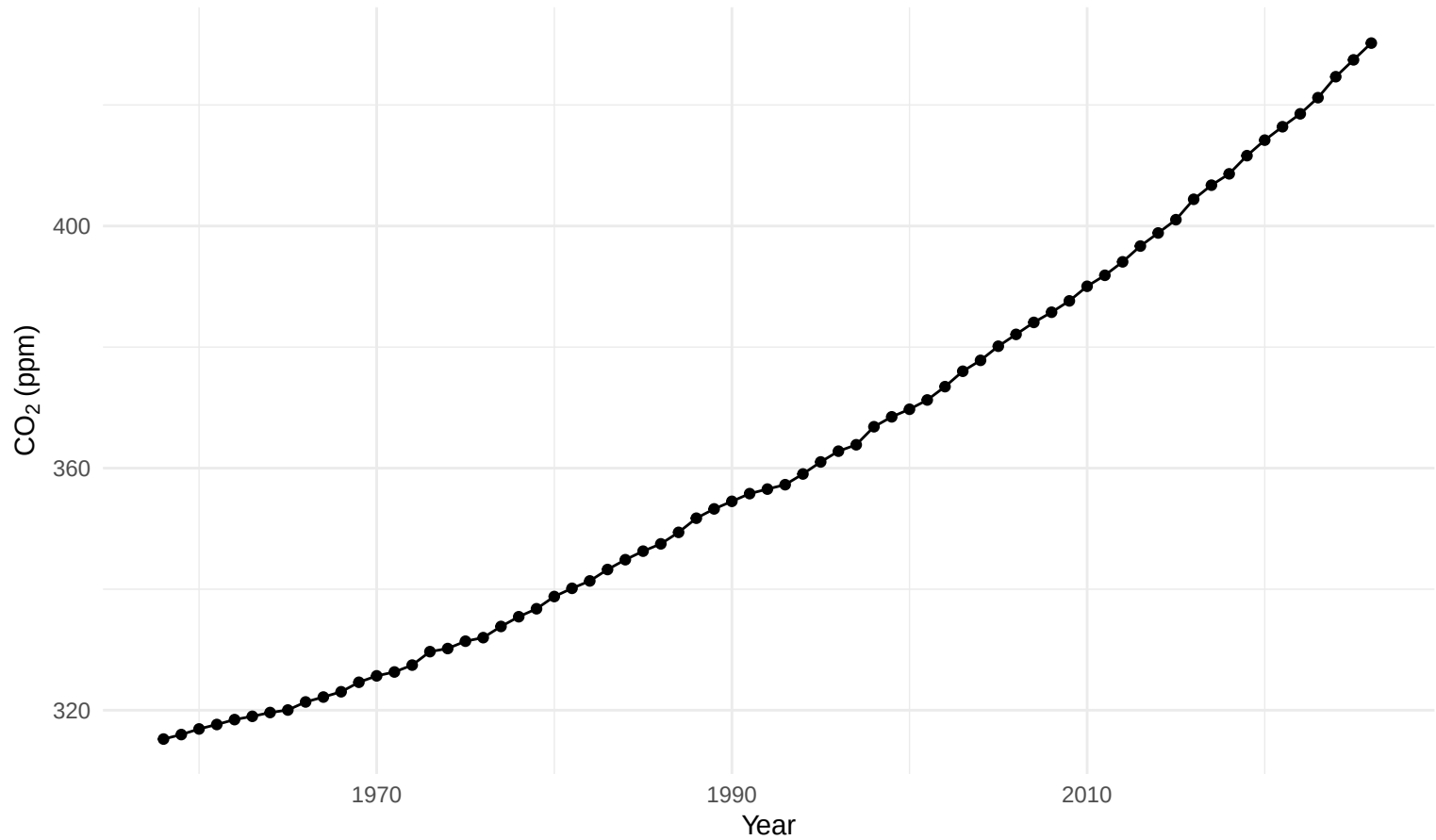
Annual average CO 2
