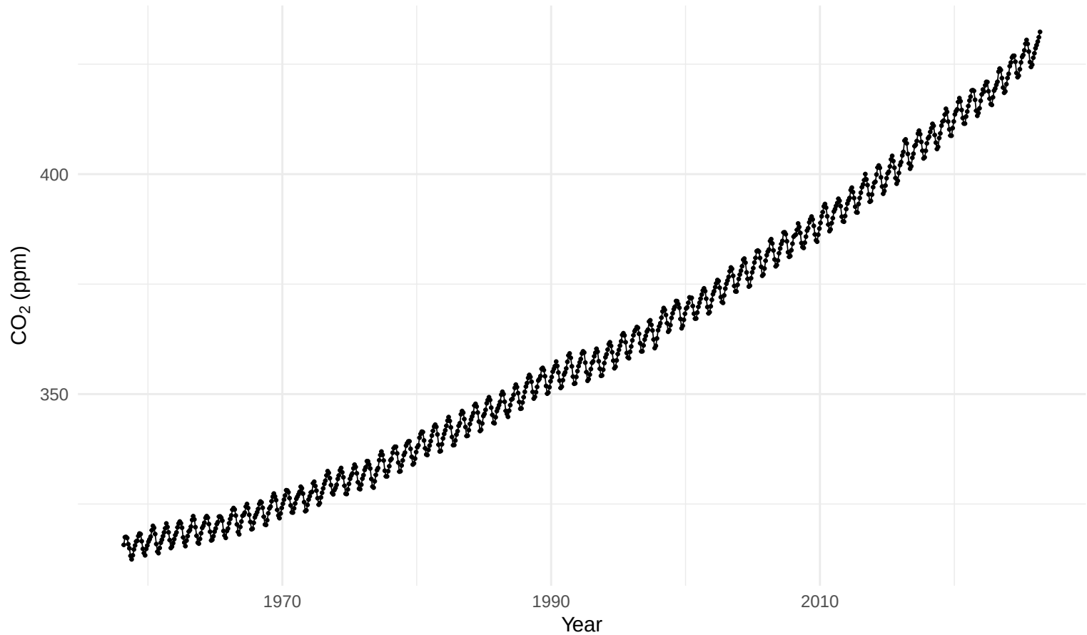
Monthly CO 2 measurements
