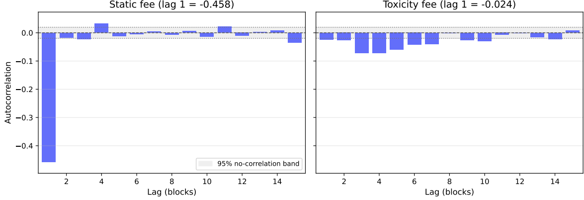
Figure 2: Autocorrelation function of end-of-block DEX log returns in the representative Model 0 seed used in Figure 1. Static fees generate a pronounced lag-1 negative spike ( -0.458 ); toxicity-based fees attenuate the lag-1 autocorrelation to -0.024 , consistent with fewer next-block arbitrage corrections.
