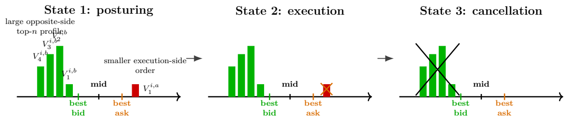
Figure 3: Schematic top- n timeline for the hypothesized spoofing mechanism. The large candidate posture forms a depth profile for the agent over several bid levels, while the smaller order rests near the opposite best quote. The construction applies symmetrically to candidate episodes with buy or sell intent. The figure shows the passive execution route; the operational reconstruction also admits an aggressive execution by the same actor.
