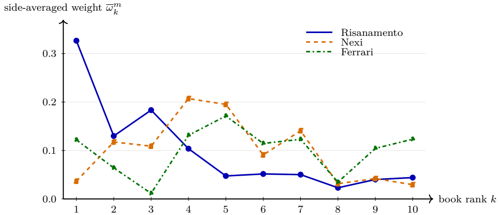
Figure 5: Empirical profiles of the top-10 depth kernel estimated on the full sample at H = 10 seconds. Each line is the arithmetic mean of the separately normalized bid and ask weights in equation (11). The mean permits one curve per instrument on a common rank axis and is used only for visualization. Surveillance metrics use the underlying side-specific kernels.
