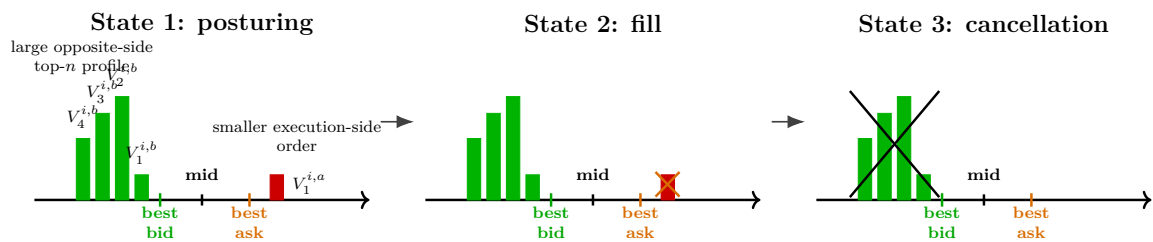
Figure 2: Schematic top- n timeline for the hypothesized spoofing mechanism. The large candidate posture forms an agent-specific depth profile over several bid levels, while the smaller order rests near the opposite best quote. The construction applies symmetrically to candidate buy- and sell-intent episodes. The figure shows the passive execution route; the operational reconstruction also admits an aggressive execution by the same actor.
