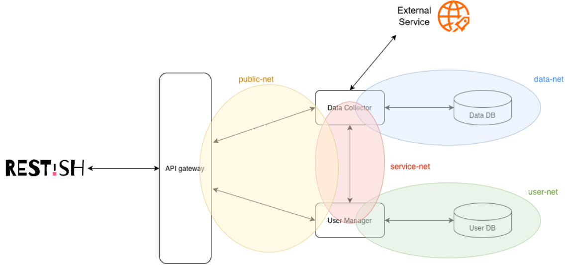
Figure 1: Architectural diagram of the Flight Data Manager system.
