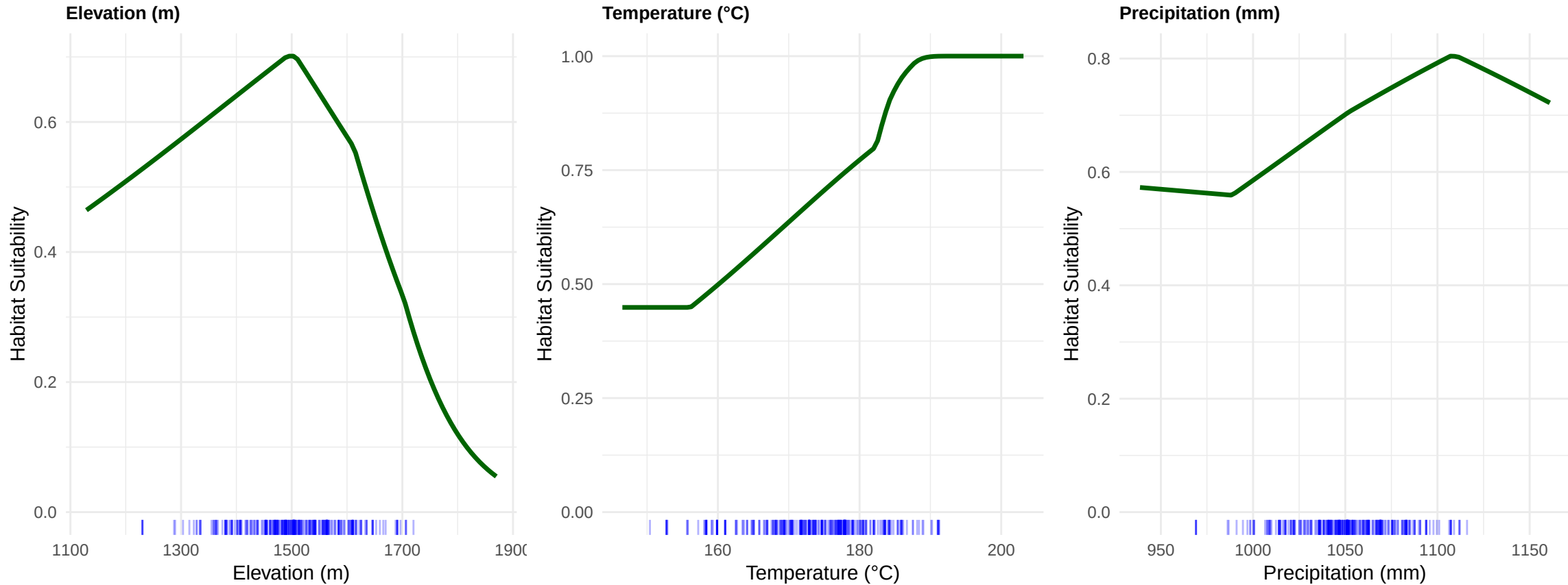
Figure 6. Response Curves for Key Environmental Variables
