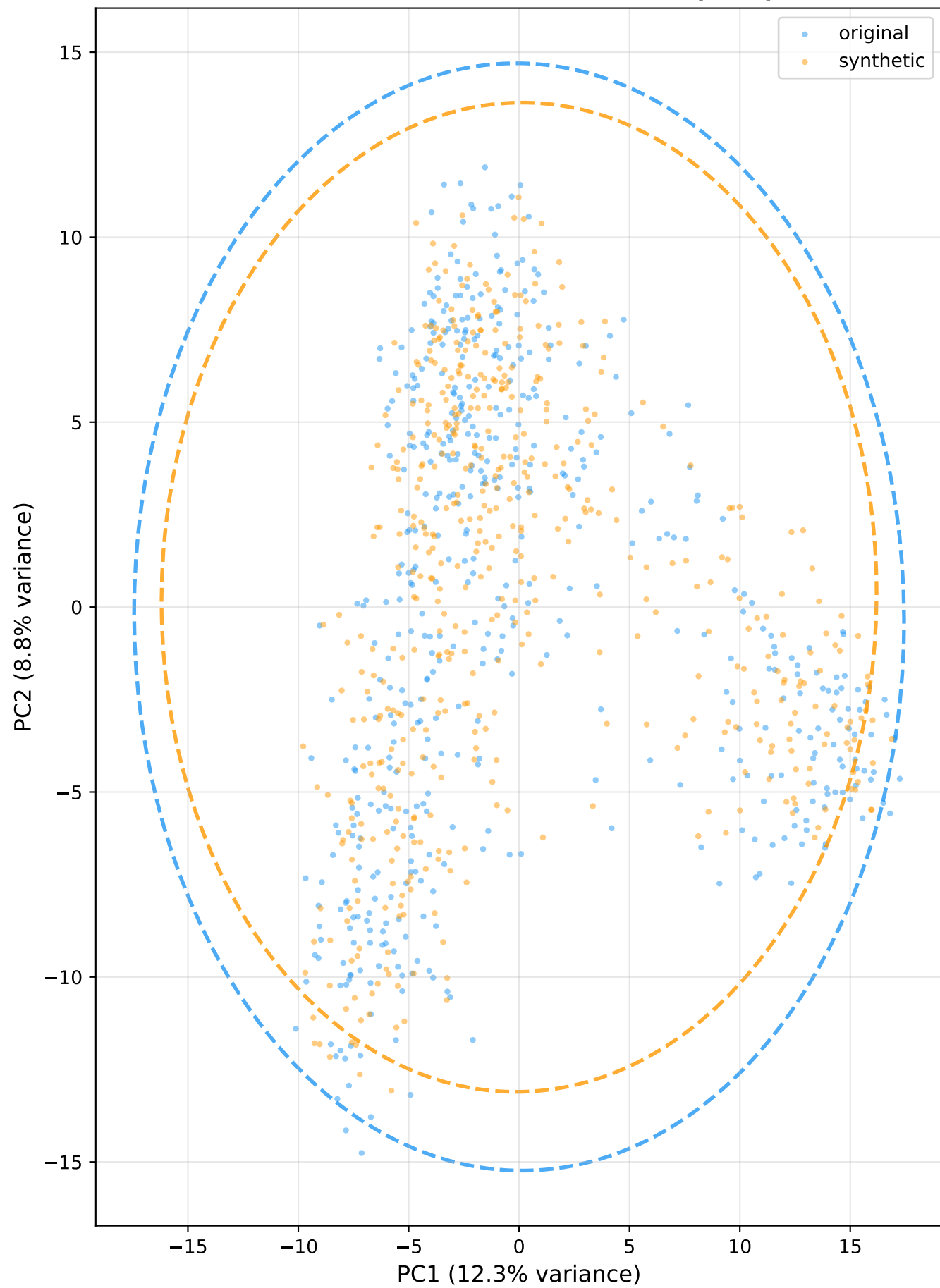
DINOv2 Feature Distribution (PCA)
