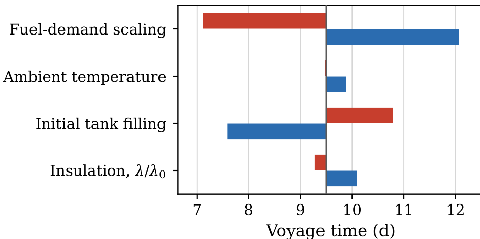
(a) Voyage time to minimum heel
