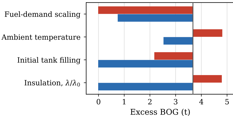
(c) Excess BOG requiring management
