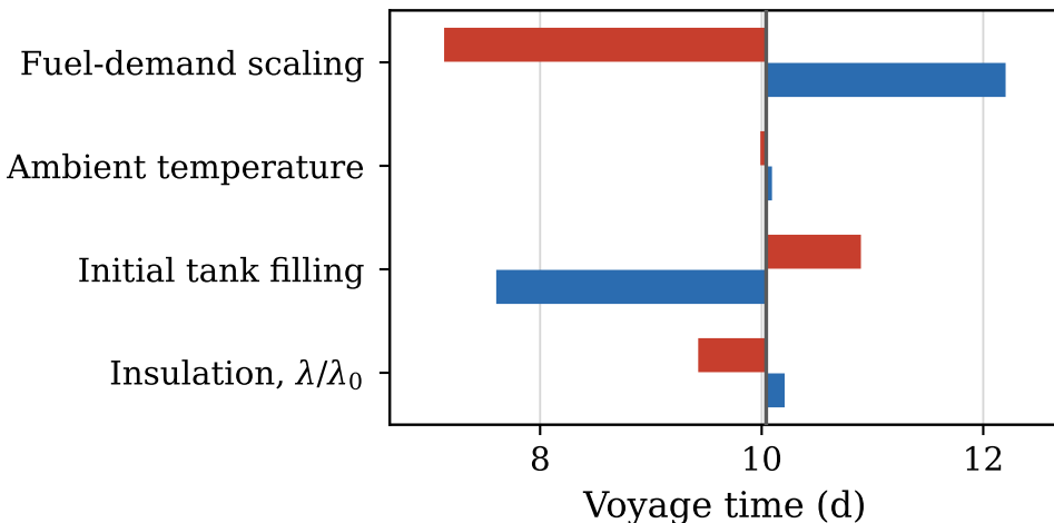
(a) Voyage time to minimum heel
