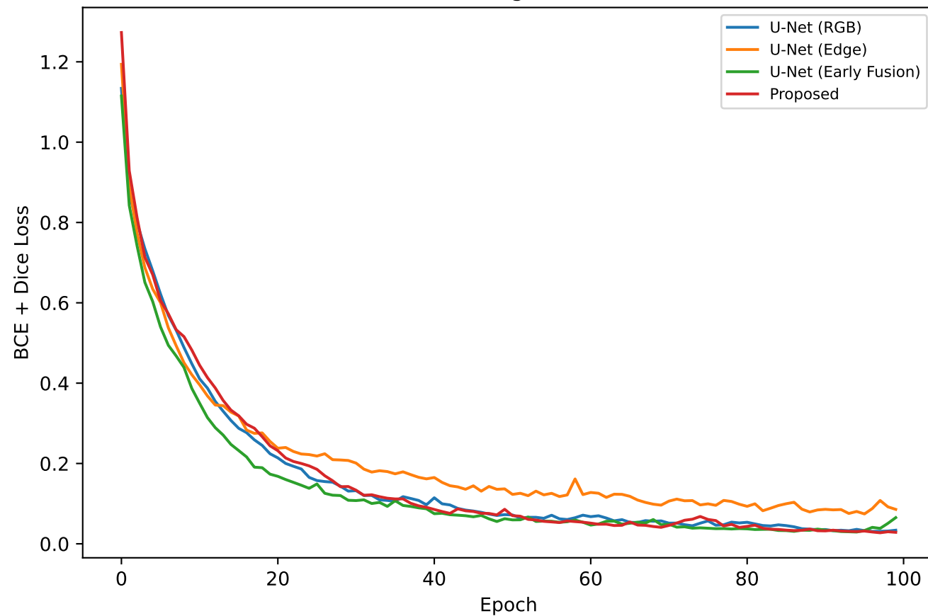
Training Loss
