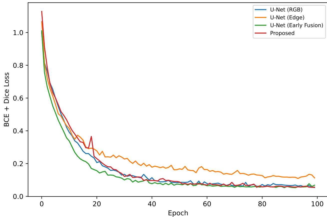
Validation Loss
