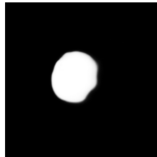
U-Net (Edge)
