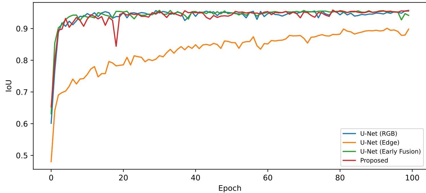
Validation IoU over Training
