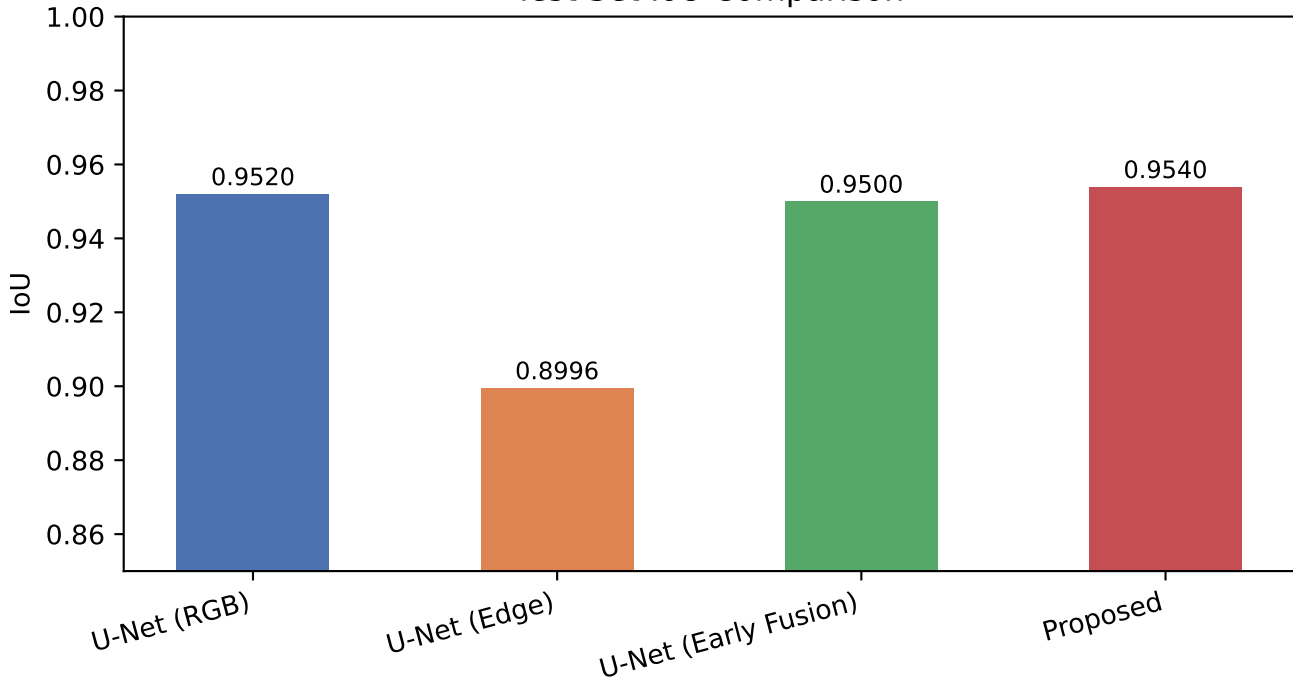
Test Set IoU Comparison
