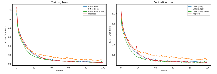
Fig. 4. Training (left) and validation (right) loss curves for all four models over 100 epochs.
