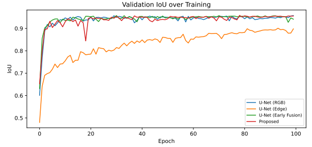
Fig. 5. Validation IoU over 100 training epochs for all four models.
