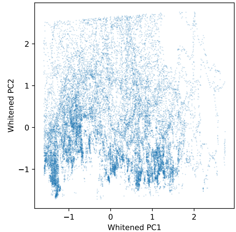
PCA-Whitened Coordinates
