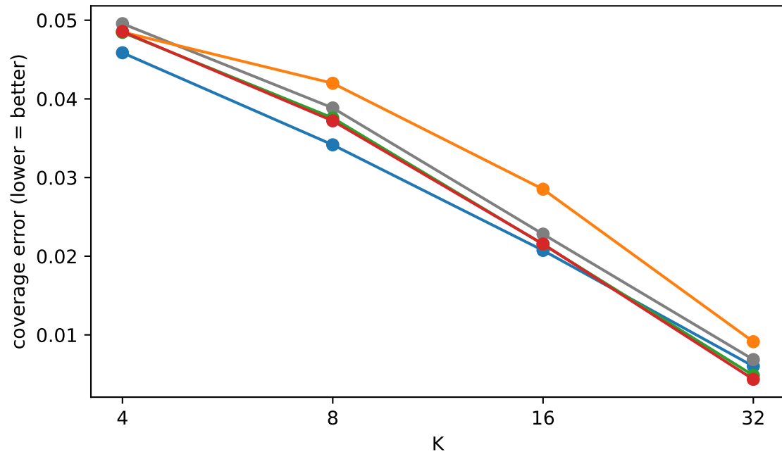
Coverage error vs K (the §5.6 crossover)
