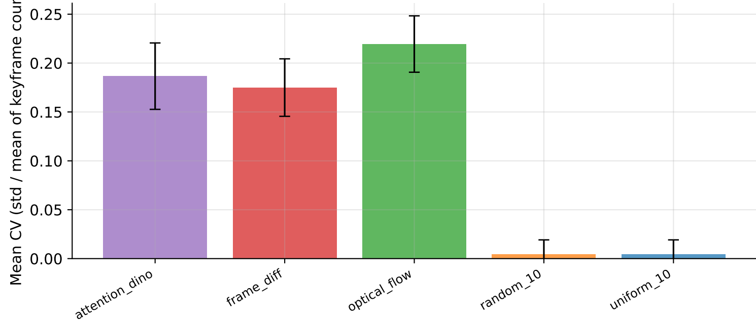
Keyframe-Count Consistency Across Tasks (CV = std / mean; lower = more consistent)
