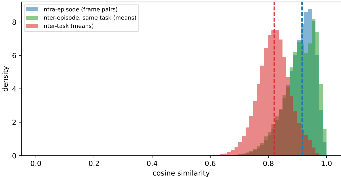
CLIP embedding similarity: within-episode vs across episodes (intra-episode tightness \gg task gap \Rightarrow selection-invariant retrieval)
