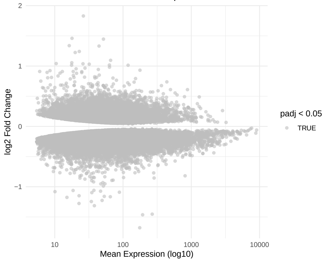
MA Plot – comp1
