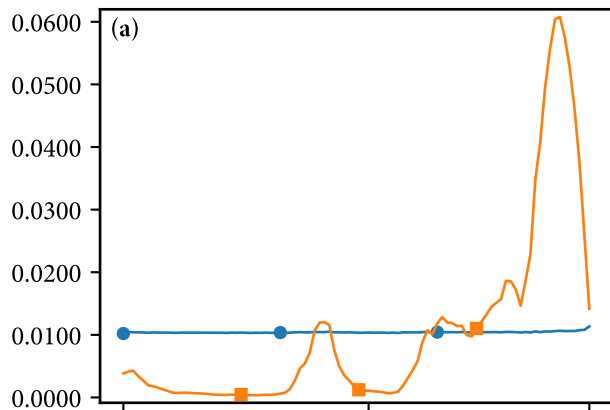
Horizon = 72-hour
