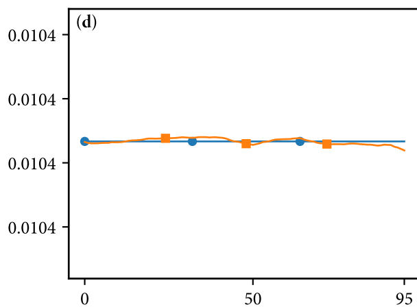
Horizon = 96-hour
