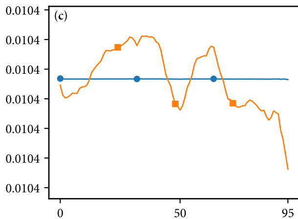
Horizon = 72-hour
