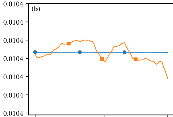
Horizon = 48-hour
