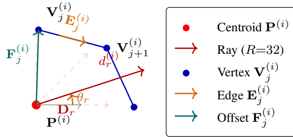
Figure 3.4. RayCast representation of a cell polygon. From the area-weighted centroid P , R = 32 rays are cast at uniformly spaced angles. Each distance d_r records the nearest boundary intersection along ray r .
