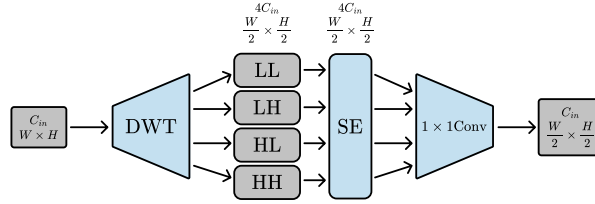
Figure 3.9. ResoConv Block Architecture
