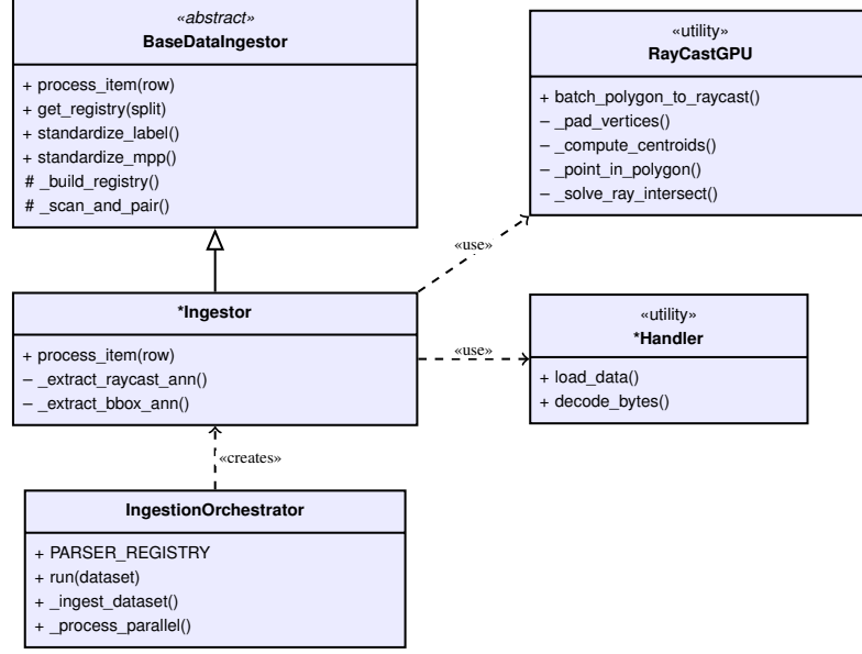
Figure 3.4. UML class diagram of the modular ingestion pipeline. BaseDataIngestor defines the shared infrastructure; concrete ingestors implement format-specific process_item logic; all converge on the unified raycast annotation format via RayCastGPU .
