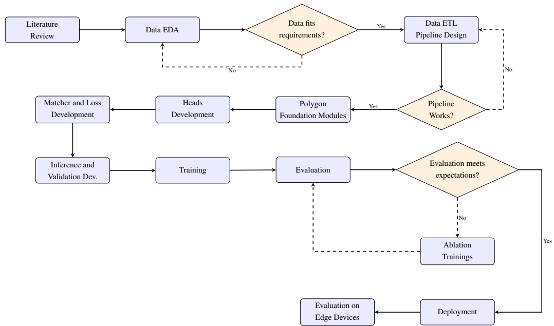
Figure 3.8. Research workflow diagram illustrating the iterative development process of the RayCastED model, from literature review and data preparation through model development, training, evaluation, and deployment.
