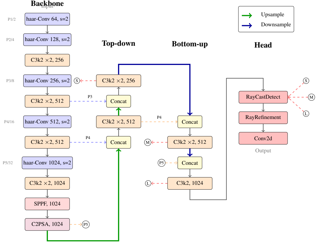
Figure 3.6. RayCastED model architecture
