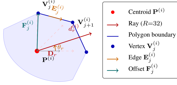
Figure 3.3. RayCast representation of a cell polygon. From the area-weighted centroid \mathbf{p} , R = 32 rays are cast at uniformly spaced angles. Each distance d_r records the nearest boundary intersection along ray r .
