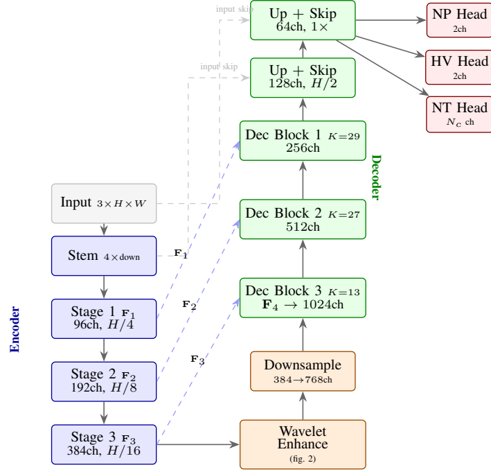
Fig. 1: Overview of the WaveLKCell architecture in a U-shaped encoder-decoder layout. The large-kernel encoder (UniRepLKNet-S) extracts multi-scale features \{F_1, F_2, F_3\} at progressively lower resolutions. The Multi-Level Wavelet Enhancement module processes F_3 through two-level Haar DWT/IDWT with frequency-specific processors (fig. 2), producing the bottleneck F_4 . The decoder upsamples through three large-kernel blocks with skip connections (dashed blue), followed by two extra upsampling stages. Three heads predict NP, HV, and NT maps.
