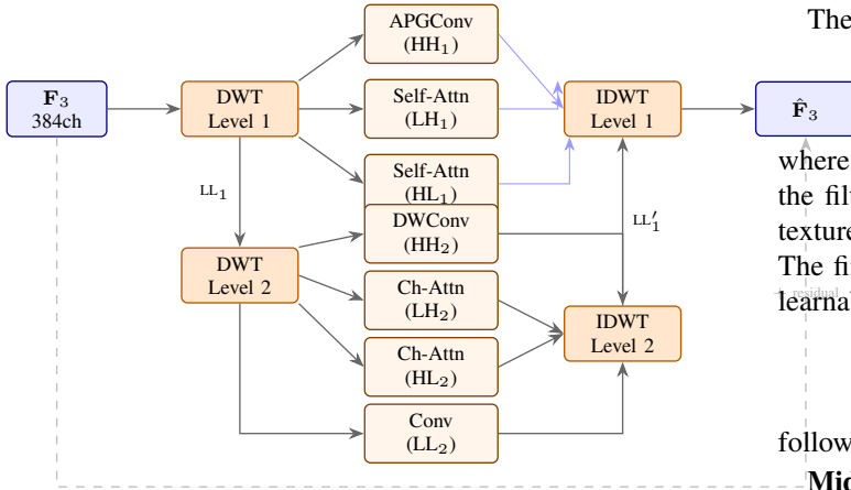
Fig. 2: Detailed view of the Multi-Level Wavelet Enhancement module. The input F_3 is decomposed by two-level Haar DWT. Each frequency sub-band is processed by a specialized module: APGConv for HH_1 (high-frequency boundaries), self-attention for LH_1/HL_1 (mid-high), channel attention for LH_2/HL_2 (mid-low), depthwise conv for HH_2 , and conv for LL_2 (lowest). Enhanced bands are reconstructed via IDWT with a residual connection.
