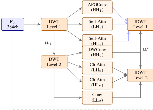
Fig. 2: Detailed view of the Multi-Level Wavelet Enhancement module. The input F_3 is decomposed by two-level Haar DWT. Each frequency sub-band is processed by a specialized module: APGConv for HH_1 (high-frequency boundaries), self-attention for LH_1/HL_1 (mid-high), channel attention for LH_2/HL_2 (mid-low), depthwise conv for HH_2 , and conv for LL_2 (lowest). Enhanced bands are reconstructed via IDWT with a residual connection.
