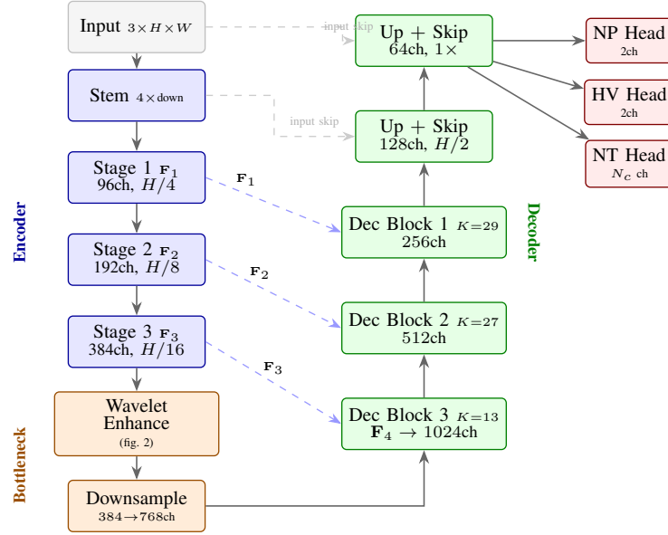
Fig. 1: Overview of the WaveLKCell architecture in a U-shaped encoder-decoder layout. The large-kernel encoder (UniRepLKNet-S) extracts multi-scale features \{F_1, F_2, F_3\} at progressively lower resolutions. The Multi-Level Wavelet Enhancement module processes F_3 through two-level Haar DWT/IDWT with frequency-specific processors (fig. 2), producing the bottleneck F_4 . The decoder upsamples through three large-kernel blocks with skip connections (dashed blue), followed by two extra upsampling stages. Three heads predict NP, HV, and NT maps.
