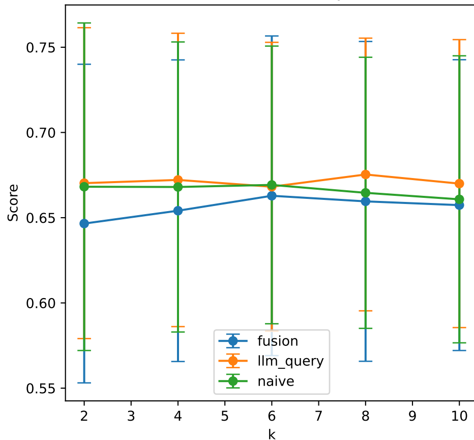
Answer Relevancy
