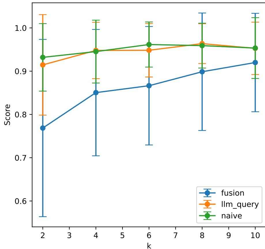
Faithfulness
