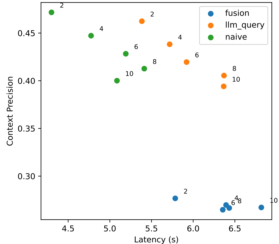
Context Precision vs Latency
