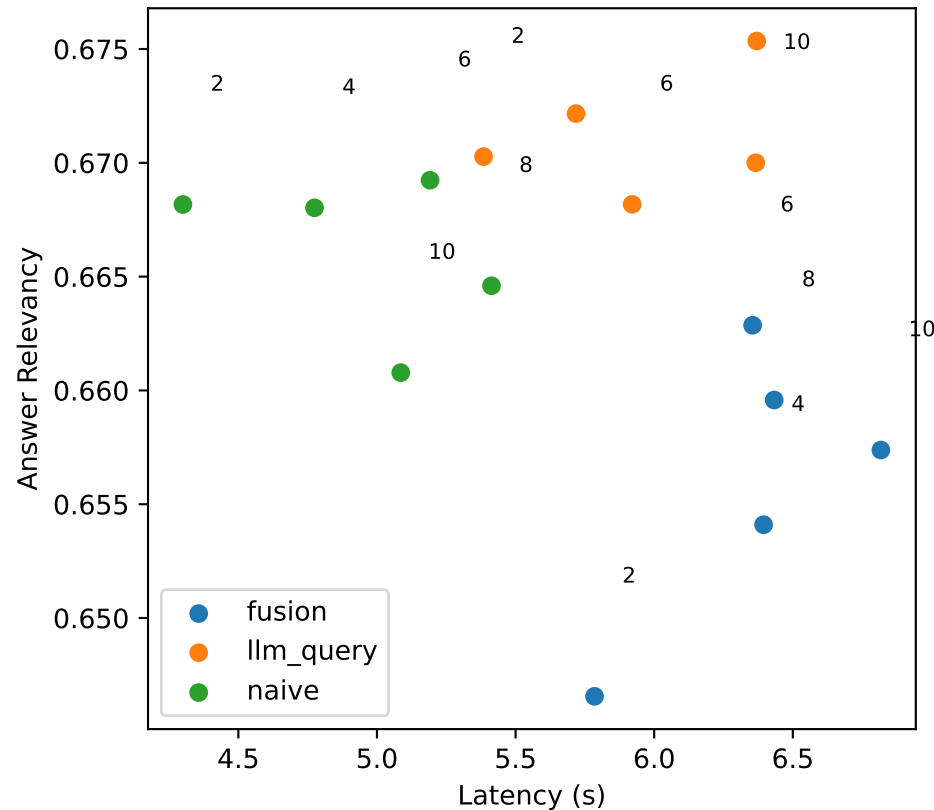
Answer Relevancy vs Latency
