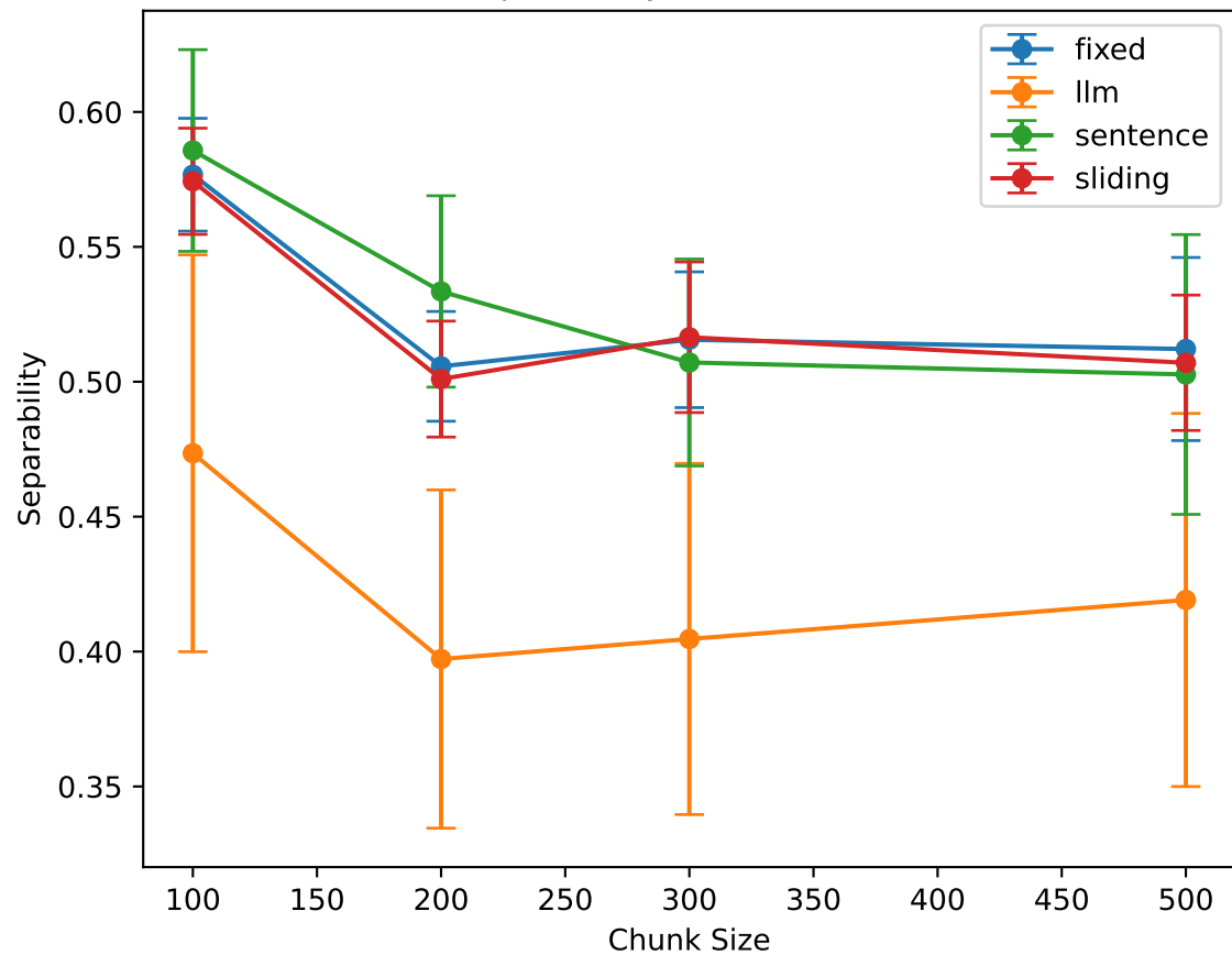
Separability vs Chunk Size
