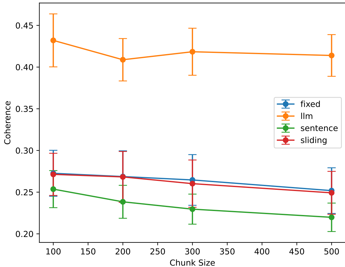
Coherence vs Chunk Size
